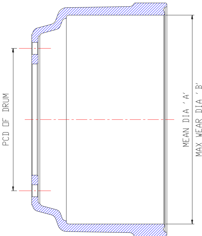
Brake Drum Dimensions
